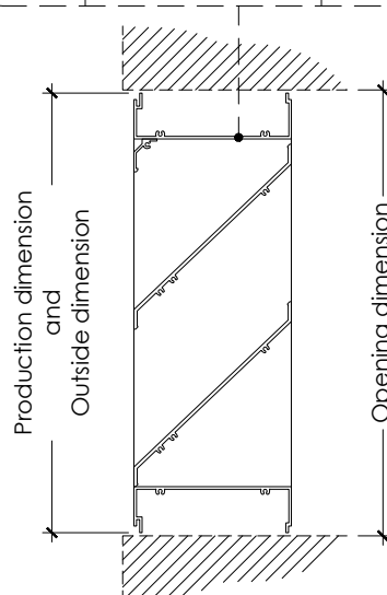
"U" frame (CU)
