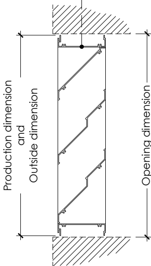
"U" frame (CU)
