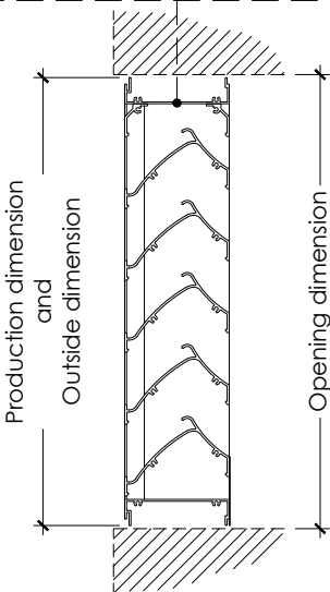
"L" frame (CL) "U" frame (CU)
