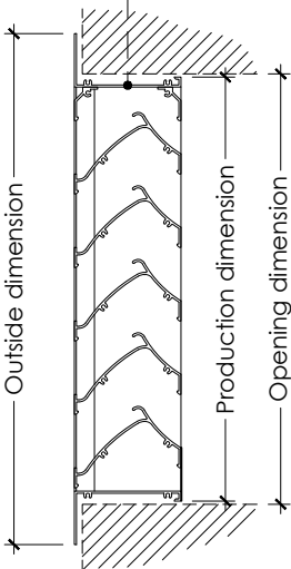
"L" frame (CL) "U" frame (CU)
