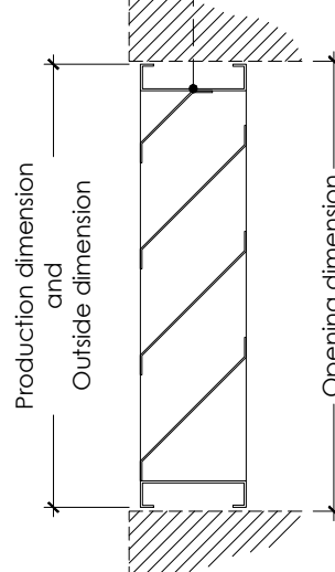
"U" frame (CU)
