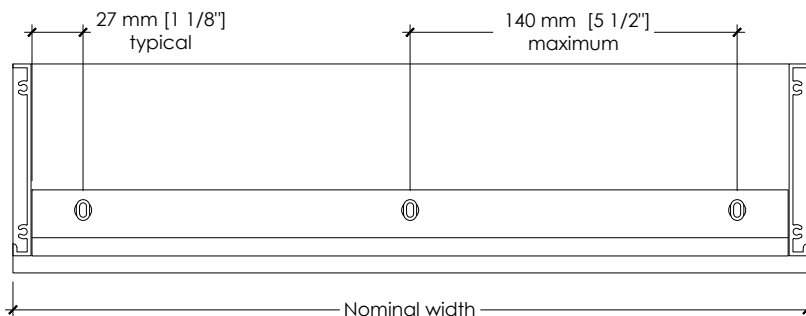
Top section
