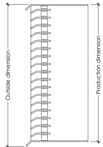
Side section
