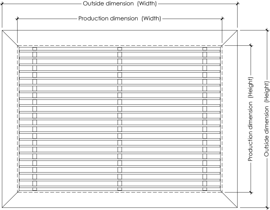
Elevation (Outside view)
