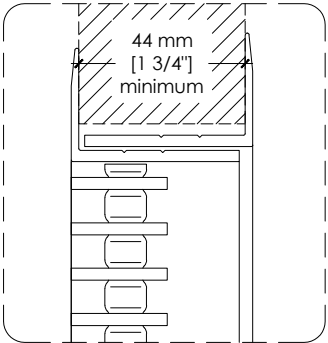
Detail Auxiliary frame (option)
