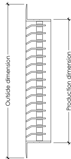
Side section
