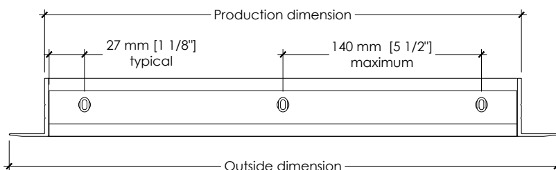
Top section
