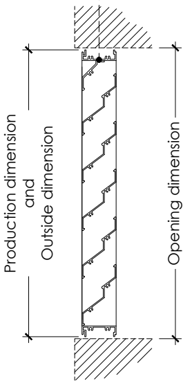
"U" frame (CU)
