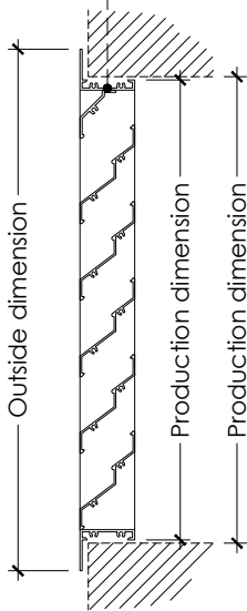
"L" frame (CL)
