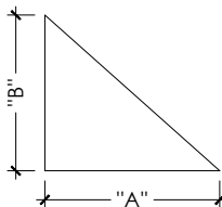
Right triangle
