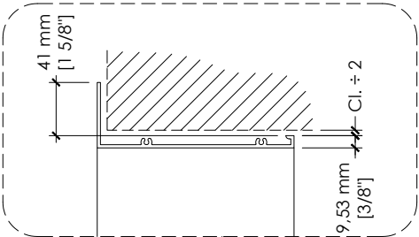
Rectangle / square
